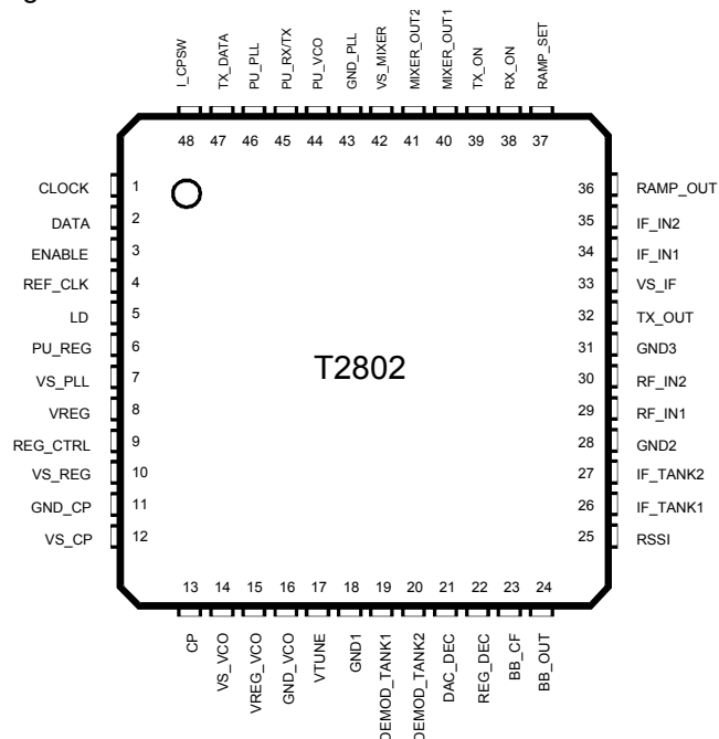
Figure 2. Pinning QFN48
